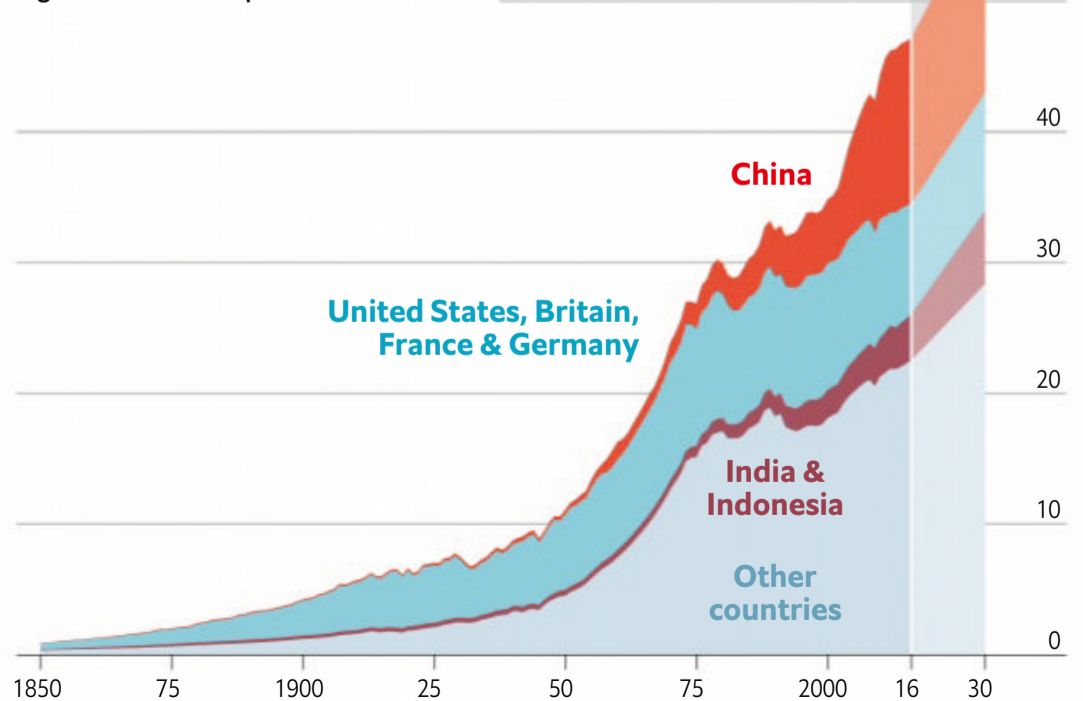
Total annual greenhouse-gas emissions Gigatonnes of CO 2 equivalent
